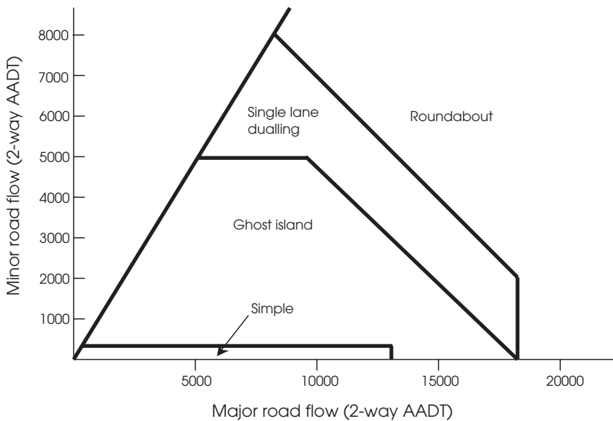
Figure 5.5 Different levels of priority intersections for various major and minor road flows in the design year.
