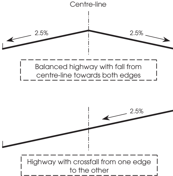
Figure 6.19 Highway crossfalls.
