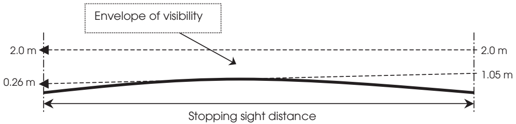
Figure 6.8 Measurement of stopping sight distance.
