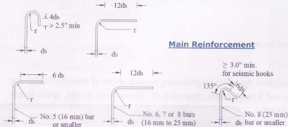
Fig. Standard bar hooks
