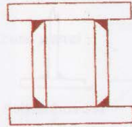
Fig. Use of groove welds at joints
