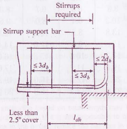
Fig. Transverse reinforcement requirements at discontinuous ends with small cover distances
