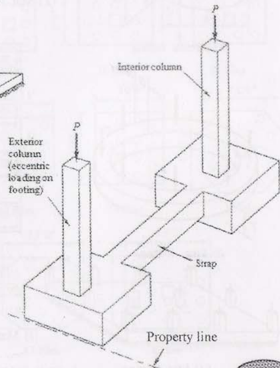
(g) Combined strap footing
