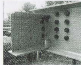
(h) Welded-bolted tee connection
