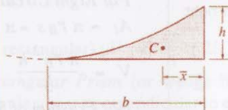
Parabolic spandrel
