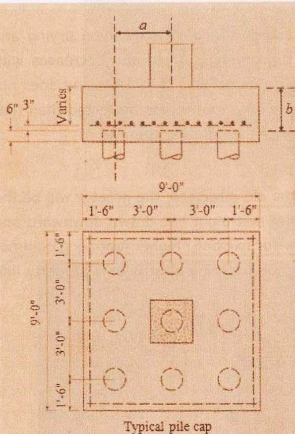
Fig. Typical single-column footing on piles (pile cap)
