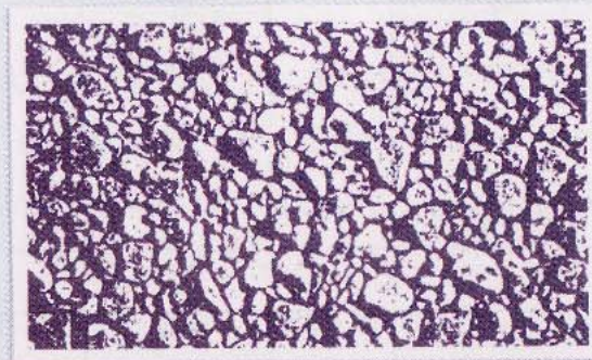
Fig. Well-graded coarse aggregate
