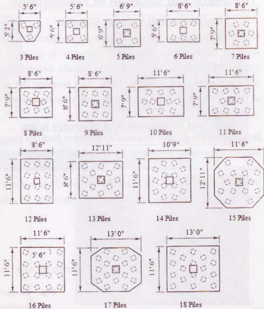
Fig. Typical configurations of pile caps
