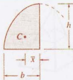
Semi Parabola
