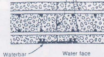
(a) Contraction joint in reservoir wall
