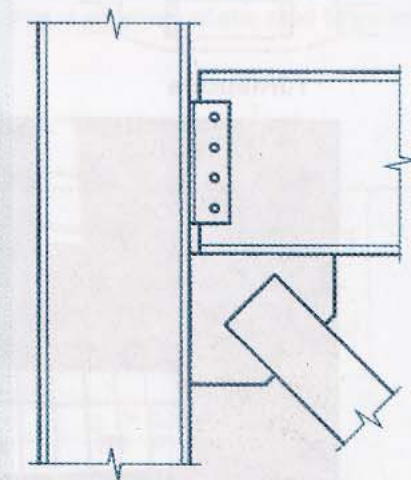
X-brace connection detail
