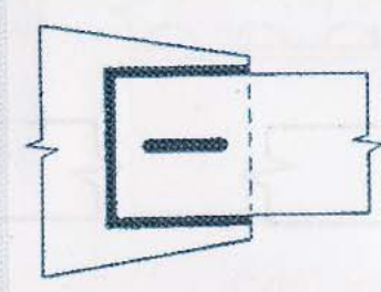
Fig. Slot and plug welds in combination with fillet welds
