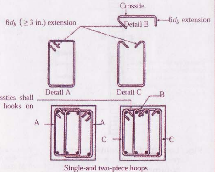
Fig. Hoop reinforcement for beams
