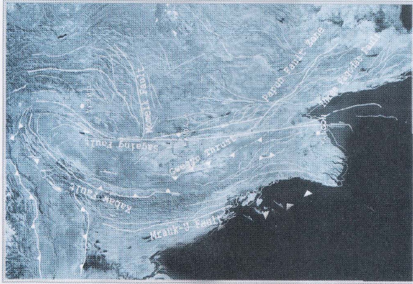
Fig. Active faults in Myanmar
