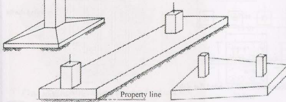
(f) Combined slab footing (trapezoidal)
