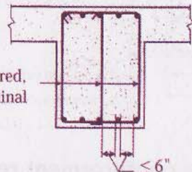
Fig. Transverse reinforcement requirements for beams
