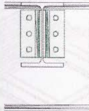
(a1) Bolted-welded double-angle connection
