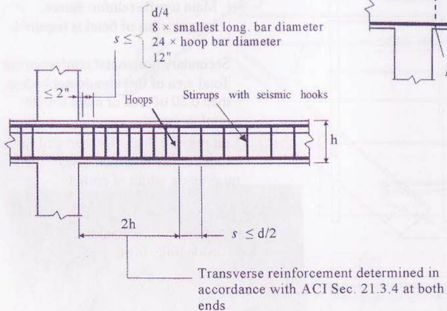
Fig. Flexural requirements for beams
