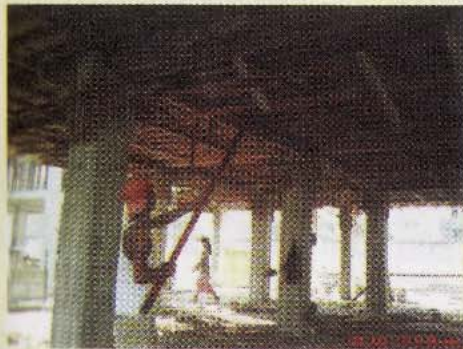
Removal of slab form
