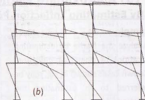
Fig. Lateral load analysis by Portal Method : (a) moments, shears, and axial forces; (b) bending moment diagram
