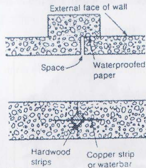
(l) Alternative designs for joints in external walls of buildings
