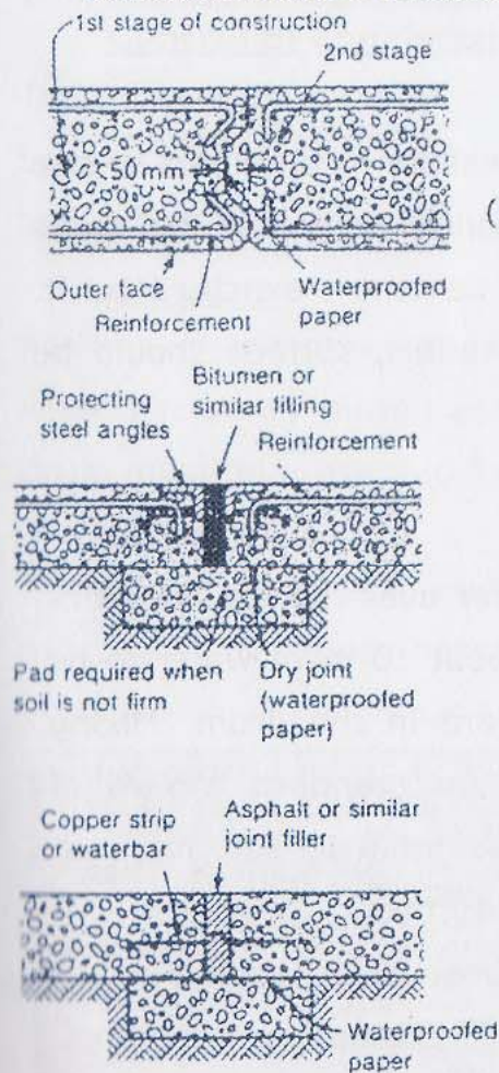
(i) Alternative designs for joints in floor laid on the ground
