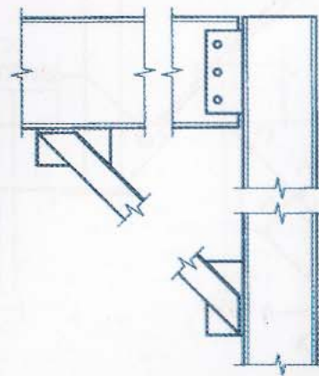
Knee brace connection detail
