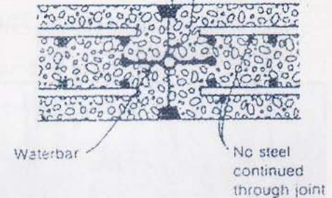
(c) Complete contraction joint in reservoir wall
