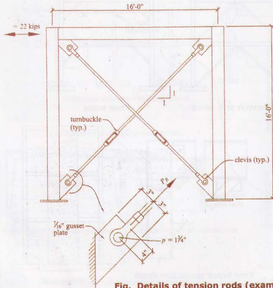
Fig. Details of tension rods (example)
