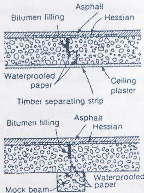
(k) Alternative designs for joints in roof slabs
