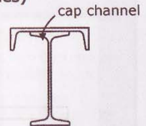
S 12x3.18 with C 10x15.3 cap channel
