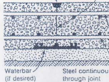
(b) Partial contraction joint in reservoir wall
