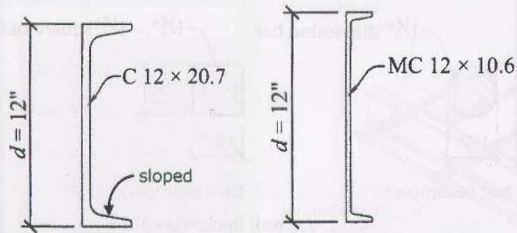
C-shape (example) (American Standard Channel)
