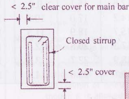
Fig. Transverse reinforcement requirements at discontinuous ends with small cover distances
