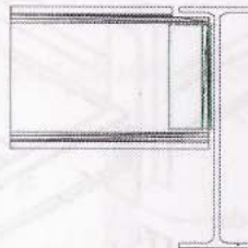
(a1) Bolted-welded double-angle connection
