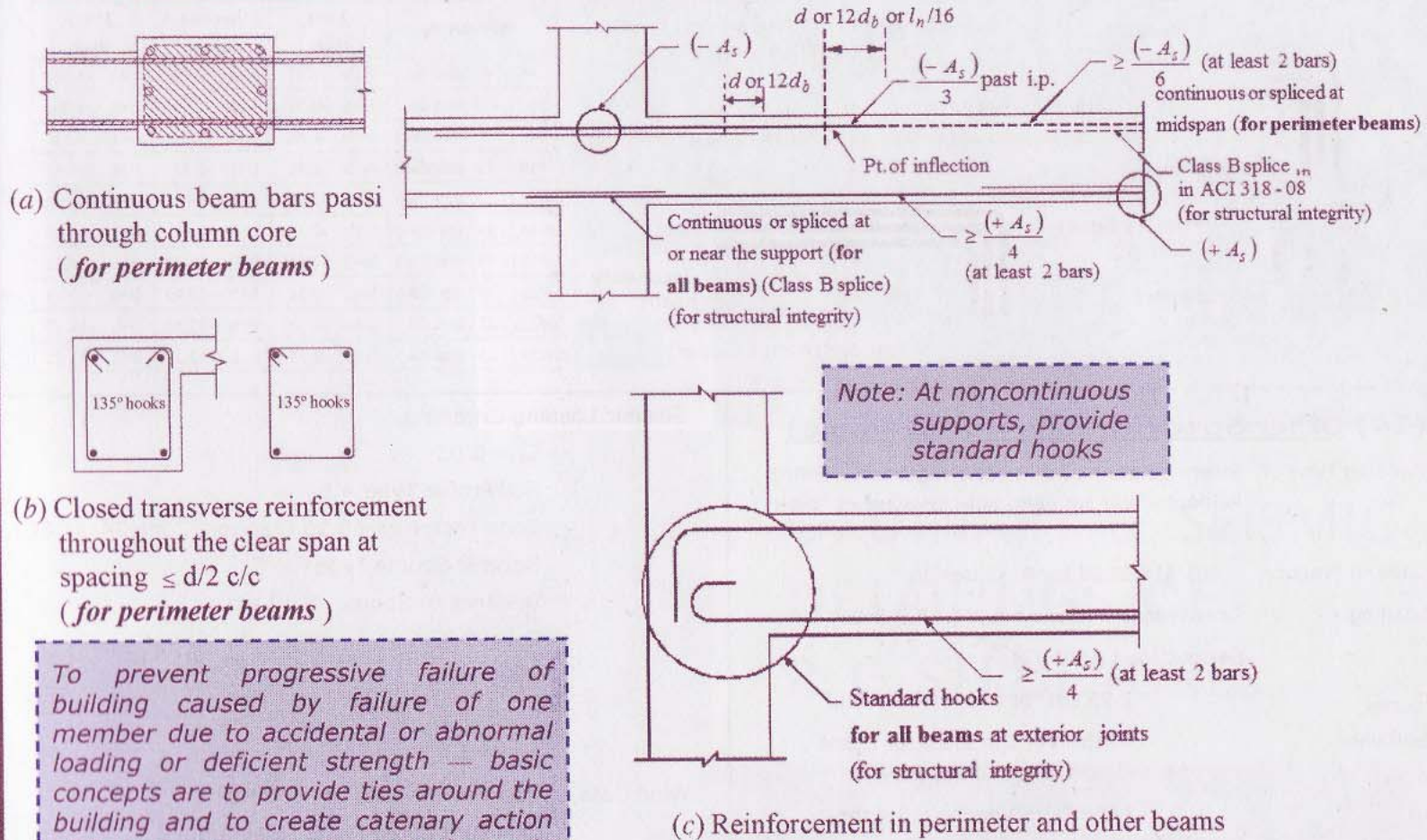
Fig. Reinforcement for structural integrity
