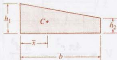
Trapezoid
