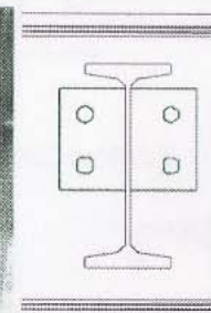
(b) Bolted shear end-plate connection
